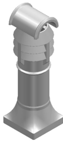
ISOMETRIC VIEW 1:20
